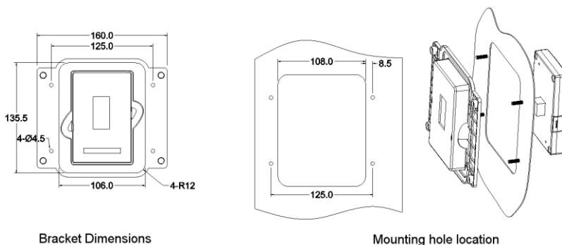
Bracket Dimensions
